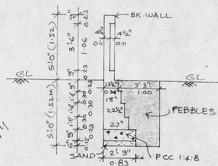
SECTION OF COMPOUND WALL & RAIN WATER STORAGE
