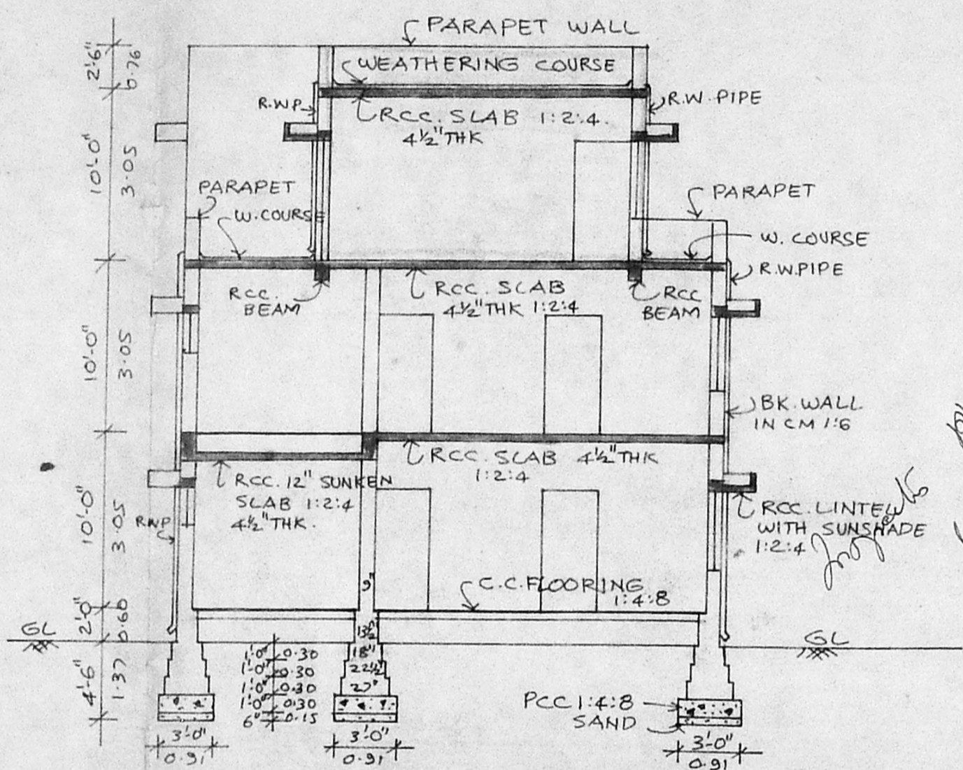
SECTION ON-AB
