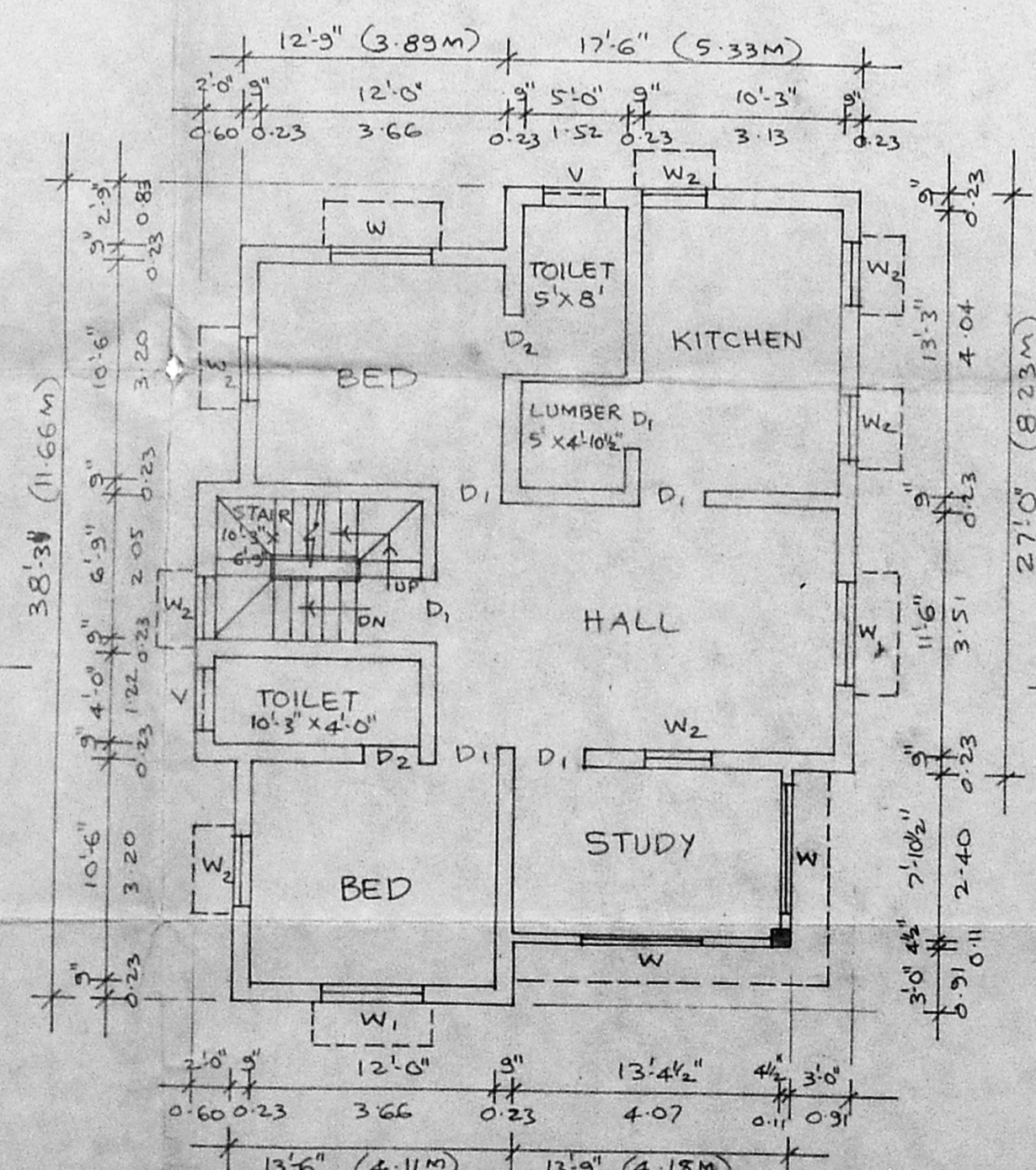
EXG. FIRST FLOOR PLAN
