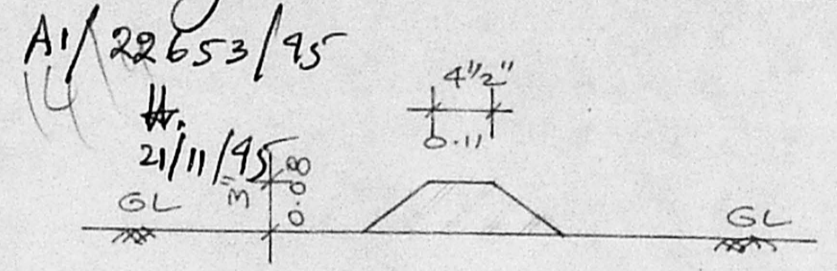
SECTION OF DWARF WALL
