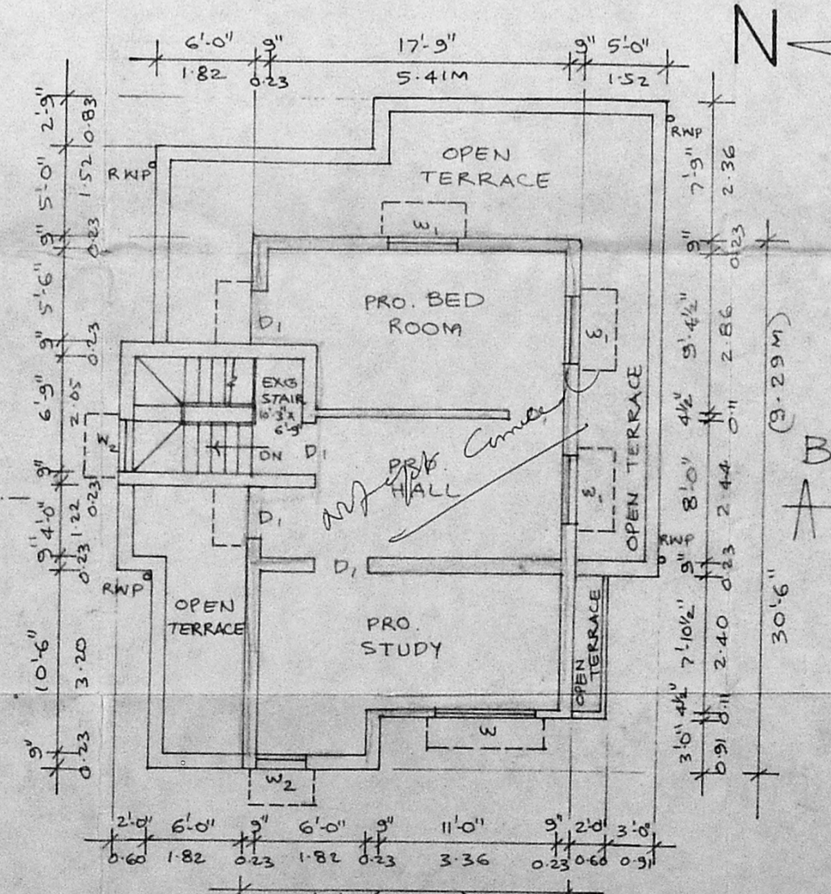
PRO. SECOND FLOOR PLAN
